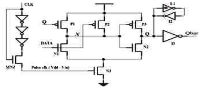
Fig.3: MHLFF
