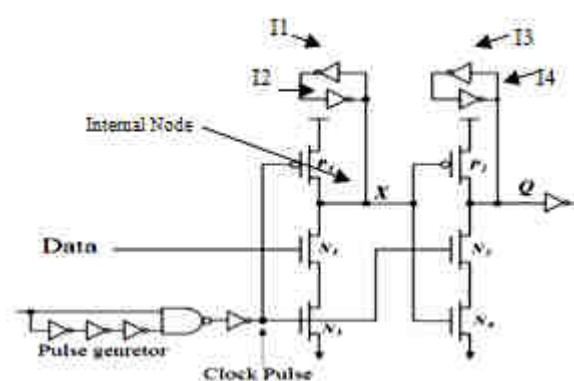
Fig.1: ep-DCO
