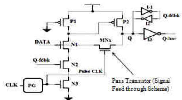
Fig.4: Proposed flip-flop
