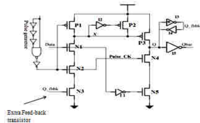
Fig.2: CDFF
